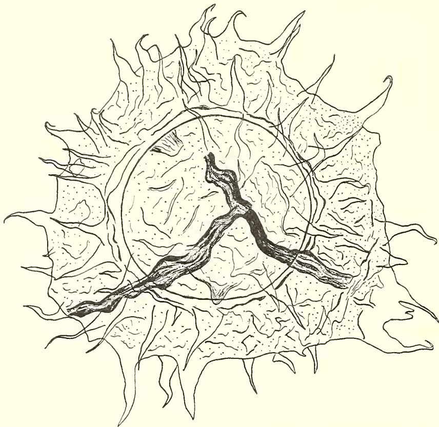
TEXT-FIG. 7. ? Spinozonotriletes cf. naumovii (Kedo), camera lucida drawing, \times 500 .
